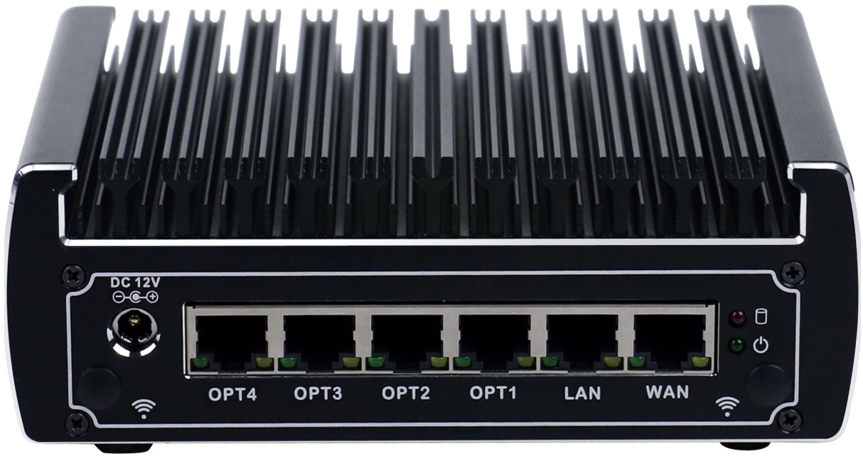
Front View
